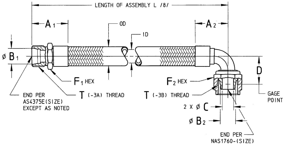
FIGURE 1 - HOSE ASSEMBLY
